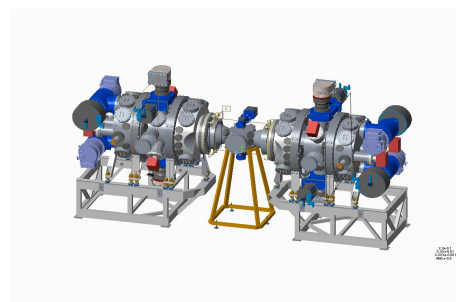
Figure 4b: Upstream and downstream UHV vacuum chambers for CRYRING with gas jet interaction chamber at the centre.
