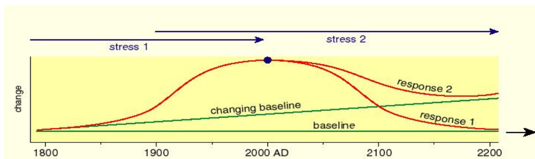
Figure. 4 Conceptual diagram illustrating ecosystem response to increasing and decreasing stresses (from Battarbee et al, 2005)
