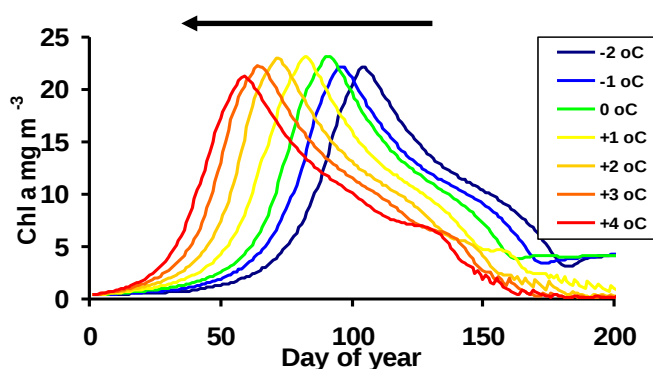
Figure 9 Effects of lake changing temperatures on algal blooms in Esthwaite Water, England (source: Elliott et al. , 2010).
