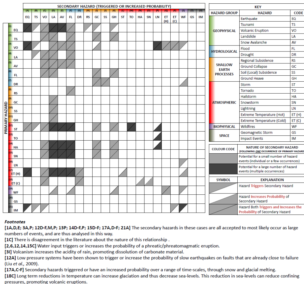
Figure 2-2 Global Hazard Interaction Framework (from Gill and Malamud, 2014). A 21 \times 21 matrix with primary hazards on the vertical axis and secondary hazards on the horizontal axis.
