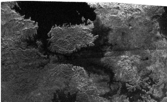
Radar image taken by instrumentation onboard Cassini of a hydrocarbon lake on the surface of Titan. The central island is ~ 150 km across. Image credit: ESA
