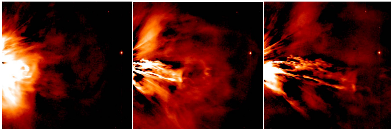
The evolution of a Coronal Mass Ejection pictured over 24 hours by the UK-led Heliospheric Imagers on the STEREO spacecraft. The bright 'star' on the right is Venus. Image credit: Jackie Davies and the HI team (Rutherford Appleton Laboratory)
