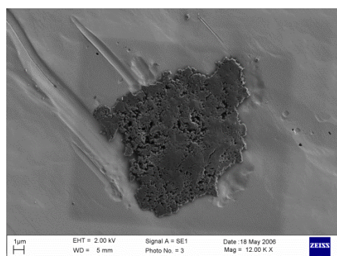
Electron microscope image of a particle from Comet Wild II embedded in aerogel then flattened onto gold foil
