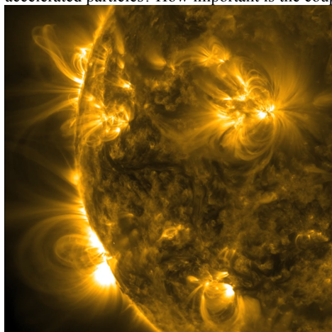
Loops above active regions of the Sun, viewed by the EUV imager of the SDO in Oct. 2012. Credit: NASA/GSFC.
