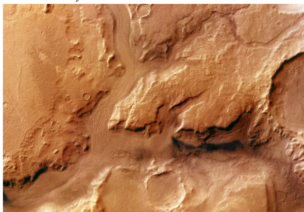
The Reull Vallis outflow channel on Mars. Credit: ESA
