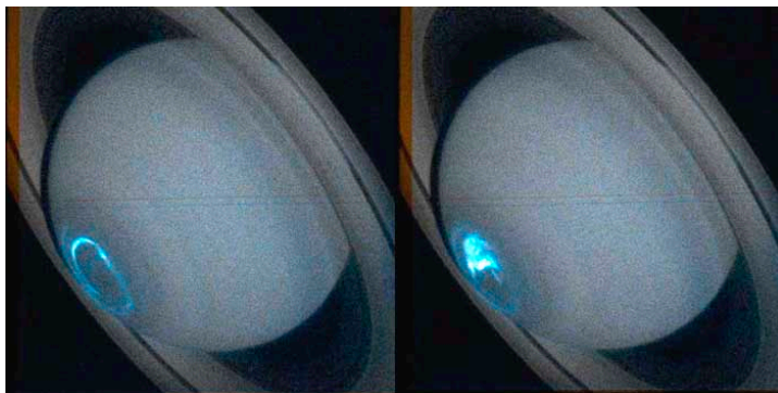
HST images of a strengthening aurora on Saturn, resulting from solar wind pressure (F. Cray et al., Nature (2005) 433, 695-696).
