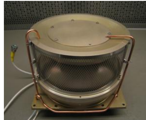
The Electron Analyser System for the Solar Wind Analyser on Solar Orbiter, currently being built at MSSL. Image credit: MSSL.
