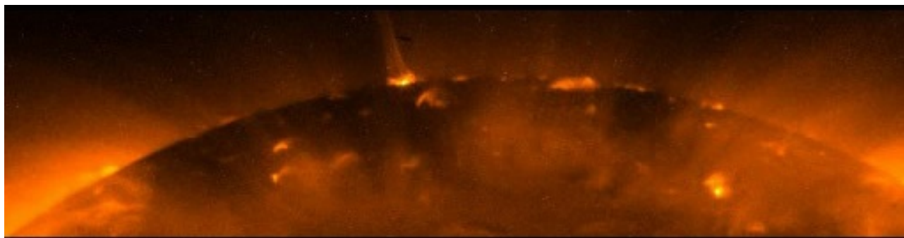
X-ray jets seen at the north pole of the Sun by the X-ray telescope onboard Hinode, in response to newly emerging magnetic fields reconnecting with the background field. Credit: Hinode X-Ray Telescope.
