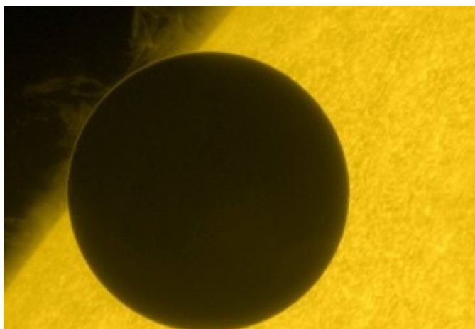
The transit of Venus in 2012, captured by Hinode. Credit: JAXA
