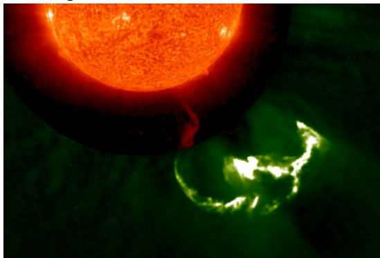
FA combination of two images from the STEREO EUV imager and solar coronagraph, showing a prominence breaking away from the solar surface in October 2012. Credit: NASA-GSFC.
