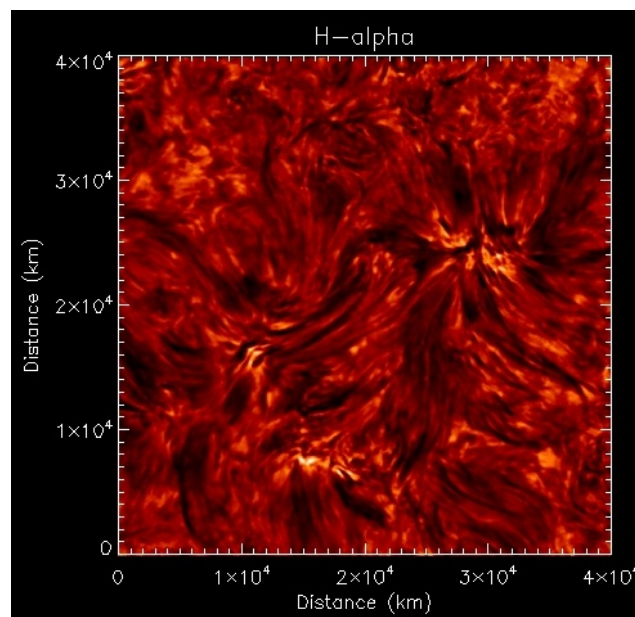
Image chromospheric spicules in Hydrogen alpha observed with ROSA showing the structure of the dynamic chromosphere down to the smallest spatial scales. Credit: Queens' University, Belfast.
