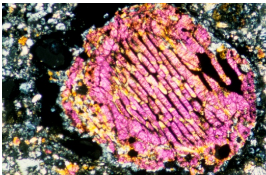
Thin section of a chondrule from a primitive meteorite, viewed through crossed polars. The chondrule has a thick rim, showing that it accumulated smaller dust grains whilst still warm. Field of view = 1 mm.
