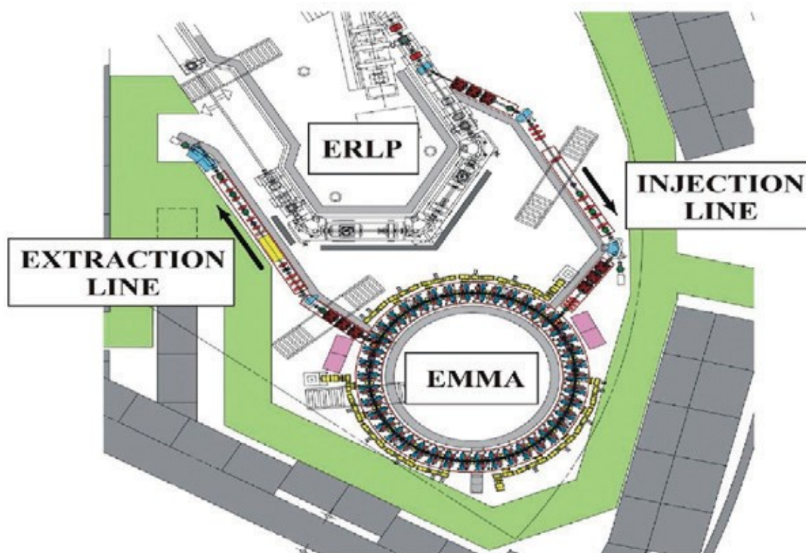
Figure 44, the ALICE & EMMA facilities
