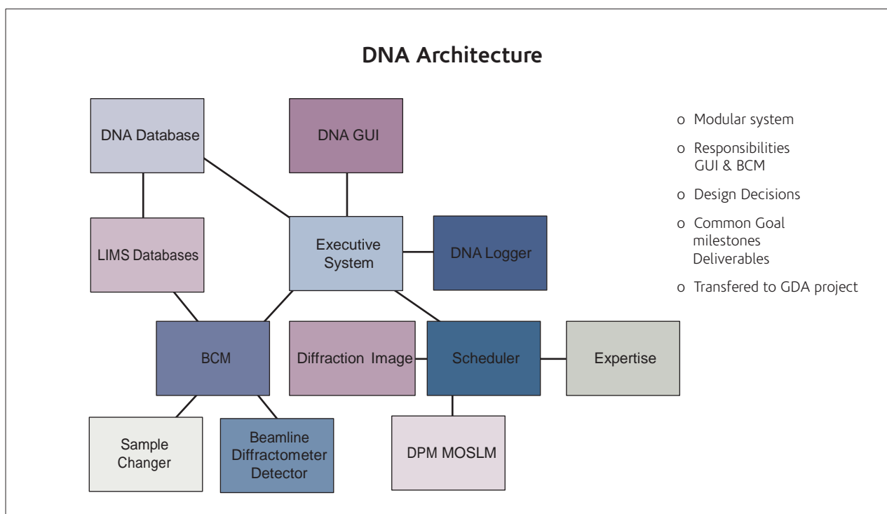
Figure 50, DNA Architecture
