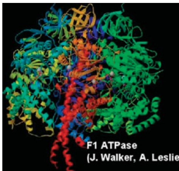
Figure 16, protein structure of F1 ATPase
