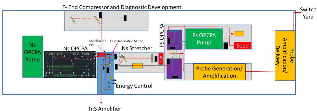
Figure 2. Approximate location within the EPAC front end for the Ns OPCPA pump laser.
