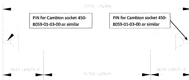
Figure 2: Diagram showing the detector lengths used in table 1.
