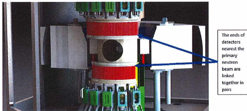
Figure 1: Detector arrangement for OSIRIS Silicon analyser upgrade. ^3\text{He} position sensitive neutron detectors in red, pre amplifier boxes in green.
