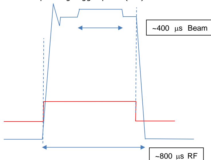
Figure 1: Typical 'closed loop' RF pulse envelope
