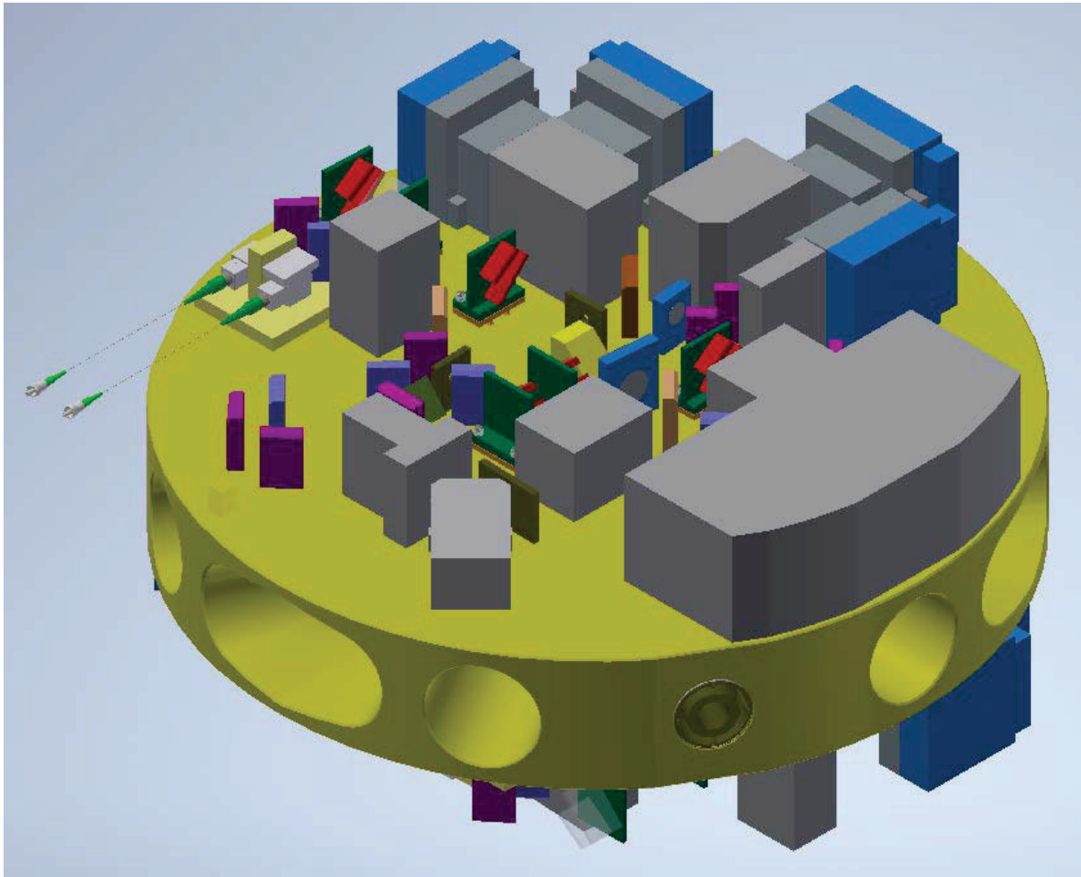
Figure 1: CAD Model of the Optical Bench showing the Zerodur baseplate fully populated on both sides.
