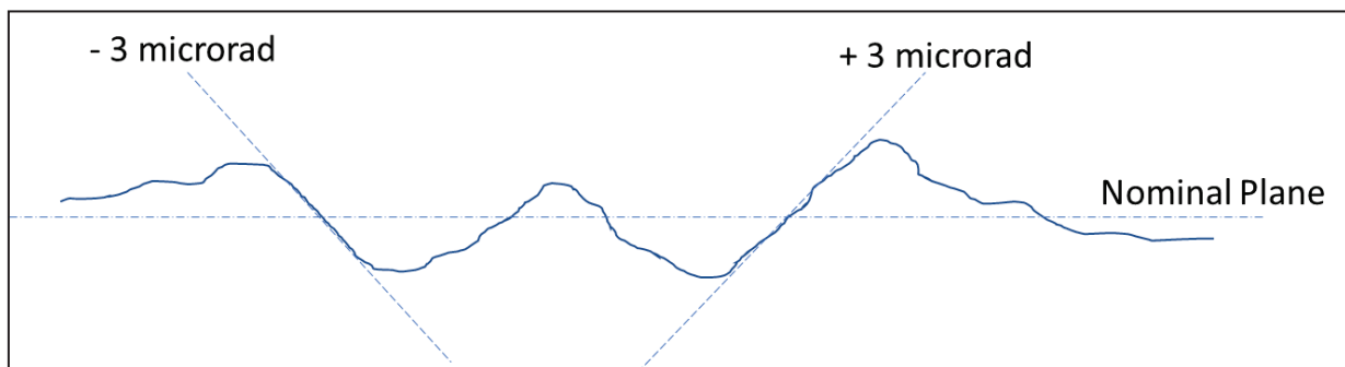
Figure 2: illustration of \pm 3 \mu\text{rad} requirement showing a surface which is within specification.
